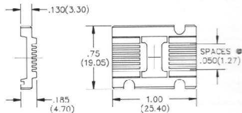
Drawing of basic 14-lead carrier without clip (others available upon request)
